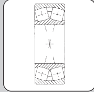
Self aligning roller bearings
